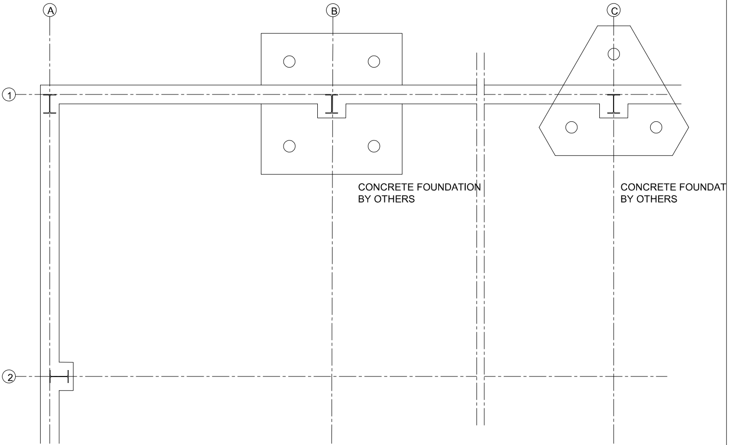
PLAN VIEW
